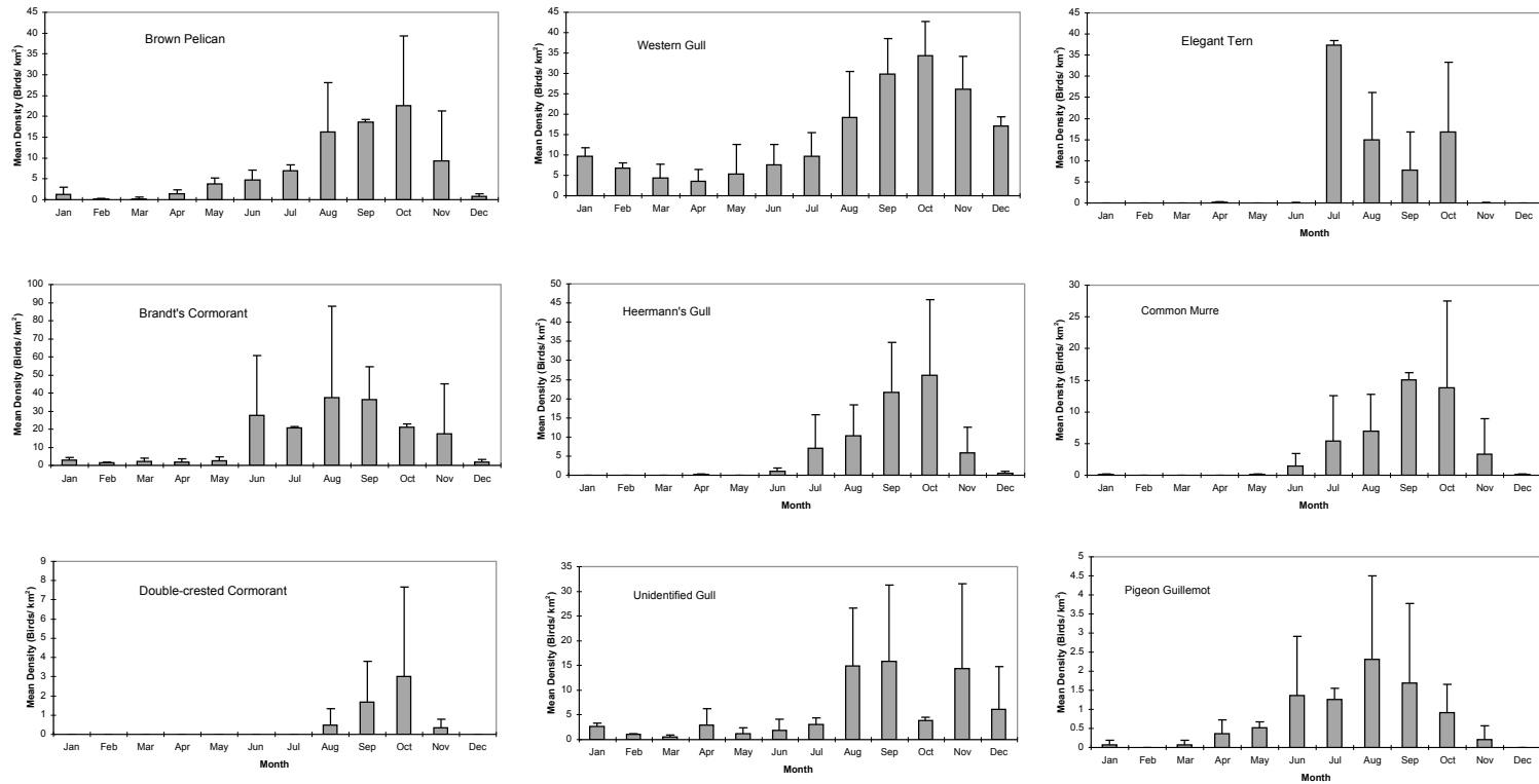
Figure 7. Mean monthly density of nine taxa of seabirds occurring in Monterey Bay primarily during fall, based on 34 surveys from 1999 to 2001. Number of surveys per month ranged from 2 to 4. Error bars are one standard deviation. Note differences in y-axis scales.
