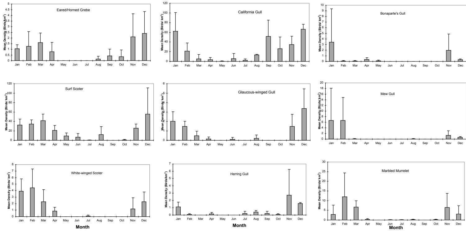
Figure 6. Mean monthly density of nine taxa of seabirds occurring in Monterey Bay primarily during winter, based on 34 surveys from 1999 to 2001. Number of surveys per month ranged from 2 to 4. Error bars are one standard deviation. Note differences in y-axis scales.
