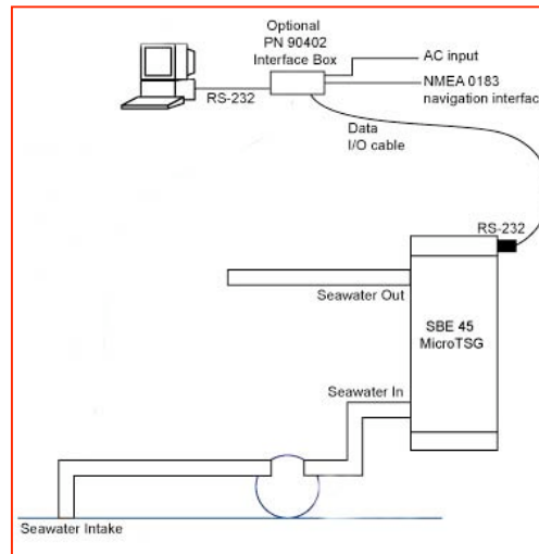
Figure 7. Operational diagram of the Sea-Bird Electronics SEACAT-SBE-19 profiler cast during CBOMP surveys.
