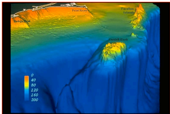
Figure 2. Cordell Bank showing surrounding seafloor along the edge of the continental shelf, Bodega Canyon to the north and east of the Bank, and other exaggerated geographic relief.
