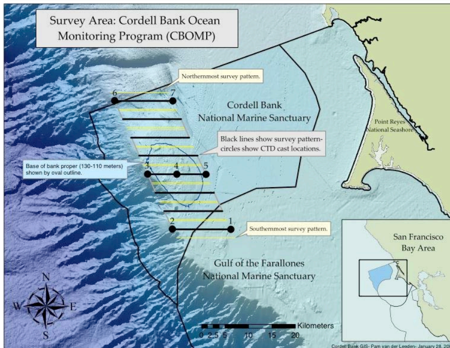
Figure 3. Cordell Bank Ocean Monitoring Program survey pattern relative to Cordell Bank, showing area covered by 13 survey patterns and positions of seven CTD casts (solid black circles).
