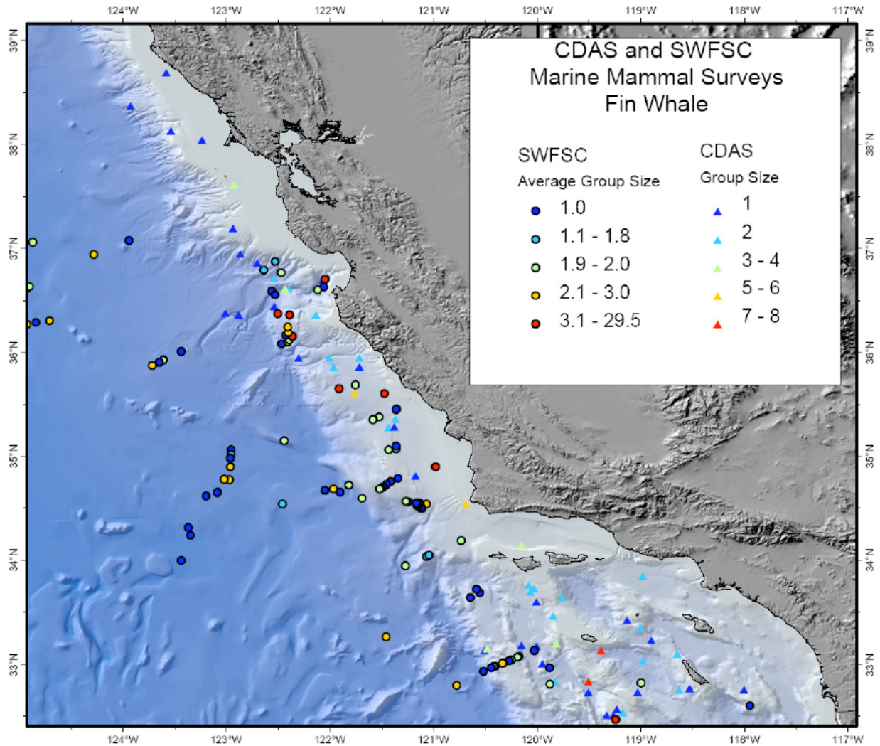
FIGURE 2. Sightings and group sizes (where available) for fin whales from Southwest Fisheries Science Center (SWFSC) ship surveys 1991-2001 and seven surveys of marine mammals compiled in the Computer Database Analysis System (CDAS) v2.1, 1975-1997 (reprinted from [4]NCCOS 2005; see Figures 6.1.2 of that report for actual transects lines surveyed by SWFSC and Figure 6.1.5 for the survey effort of the surveys in the CDAS ).
