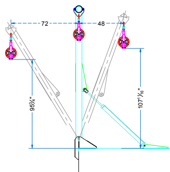
A-FRAME ARRANGEMENT
