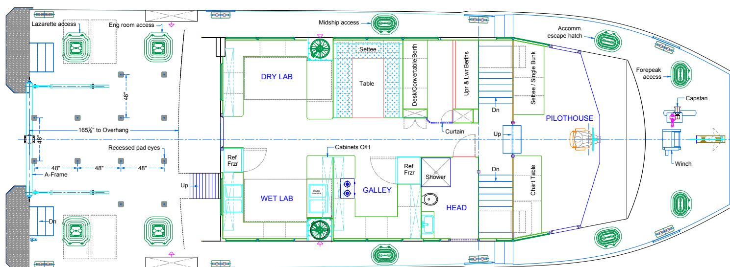
MAIN DECK ARRANGEMENT
