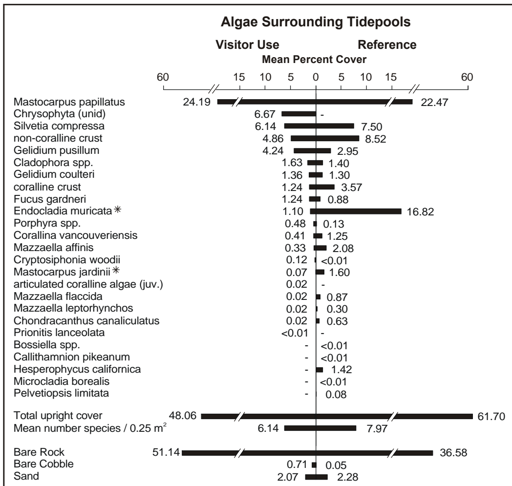
Figure 3-8. Algal and substrate cover on rocks surrounding tidepools in the visitor use and reference areas. Asterisk denotes a statistically significantly difference in abundance between areas was detected using ANOVA.
